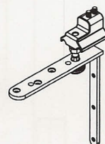
No. 21HP Pivot Set - Top Assembly
